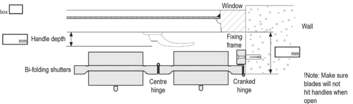
2. Frame fixed to inside of recess
