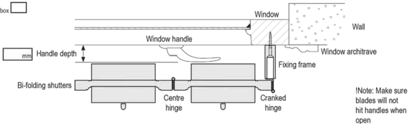
1. Frame fixed to window
