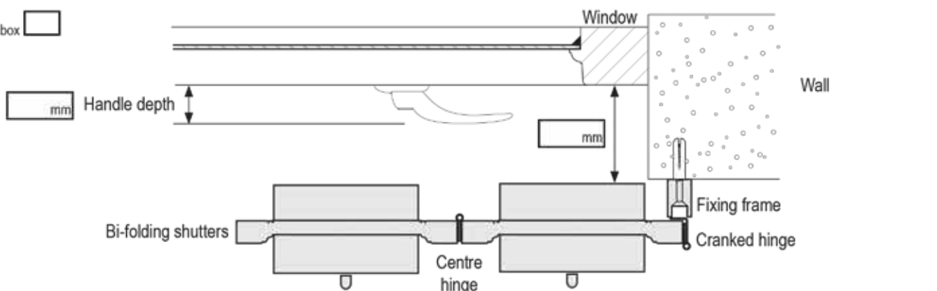
3. Frame fixed to outside of recess
